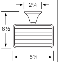
310-0.12A Wire Dish (TV)
