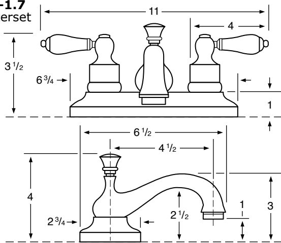
311-1.7 Centerset
