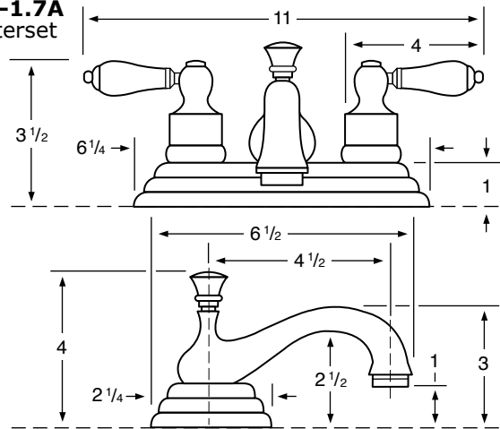
311-1.7A Curved Centerset
