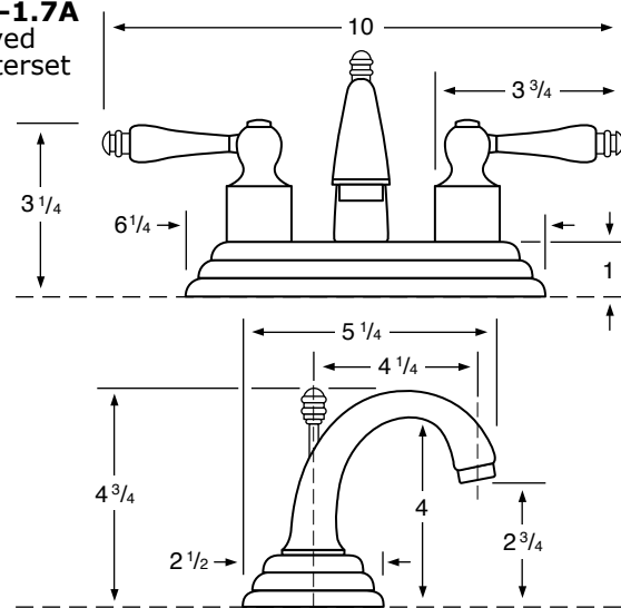
316-1.7 Centerset
